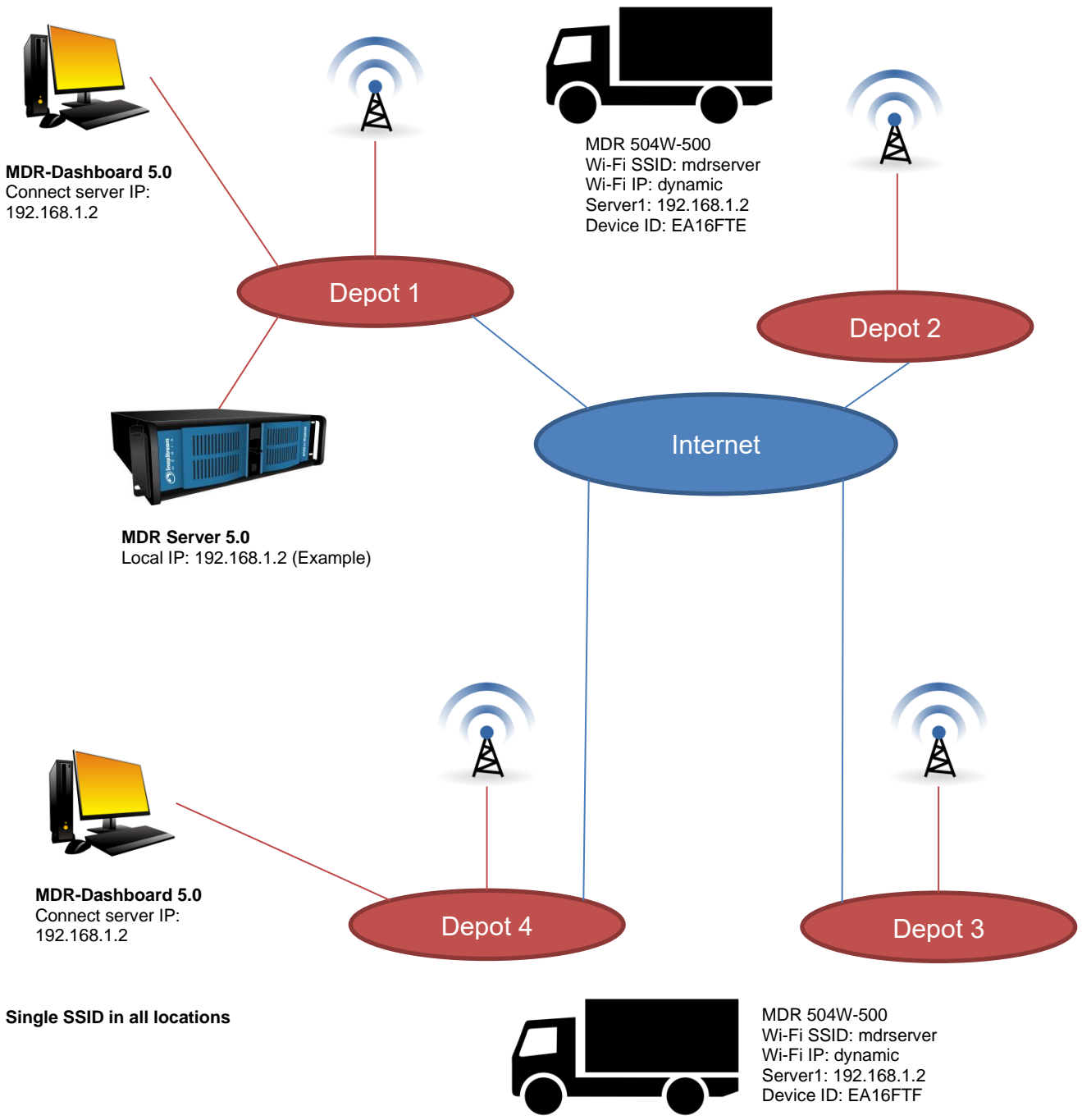
Option 3 - Wi-Fi only, multi depot, with VPN Figure 31
