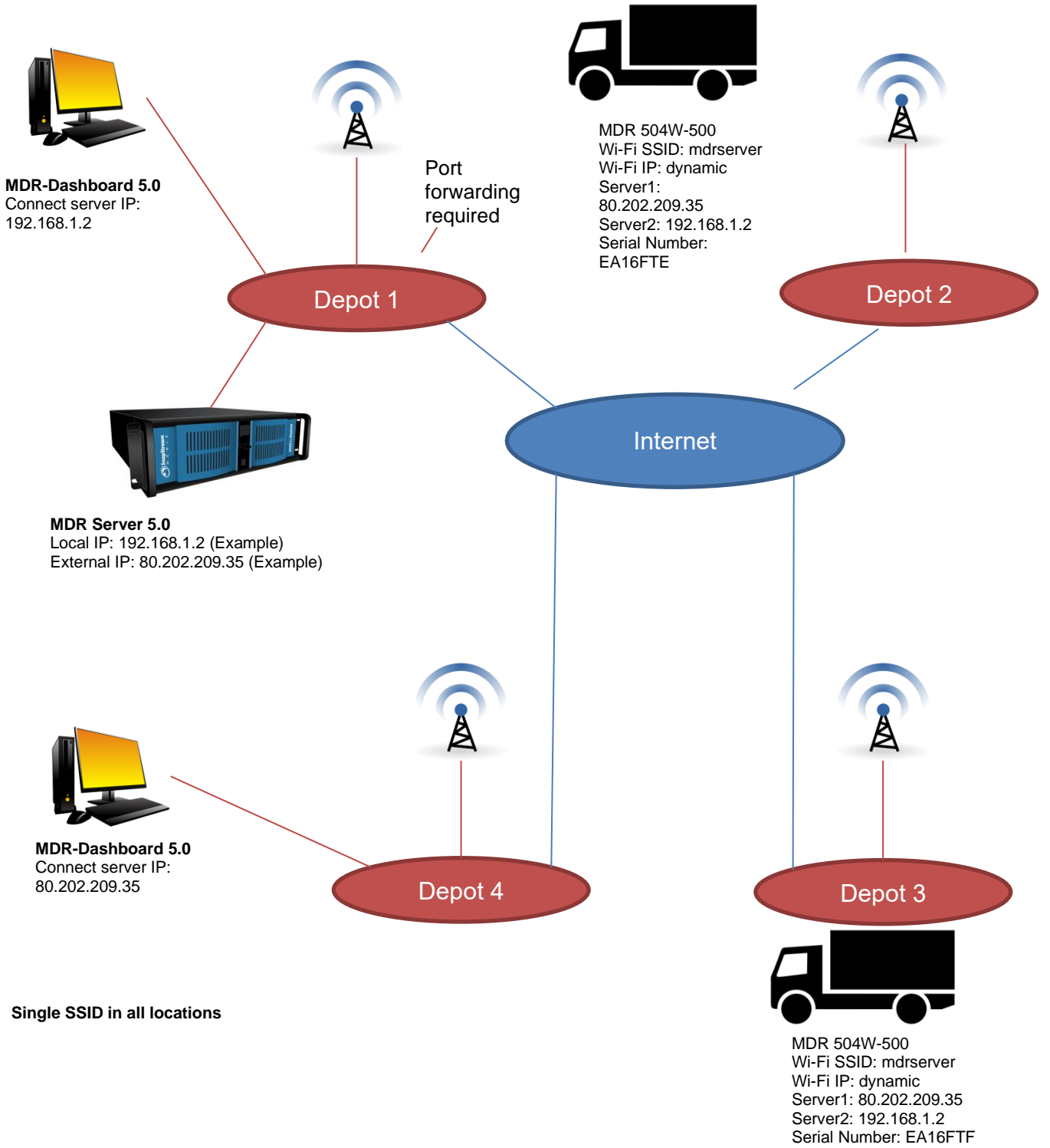
Option 2 – Wi-Fi only, multi depot, without VPN Figure 30
